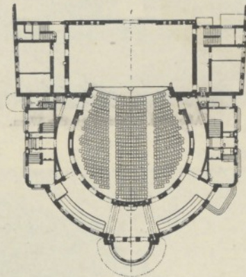
Abb. 487. Raimund-Theater. Parterre. 1:1000.
