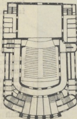
Abb. 489. Bürgertheater. Parterre. 1:1000.
