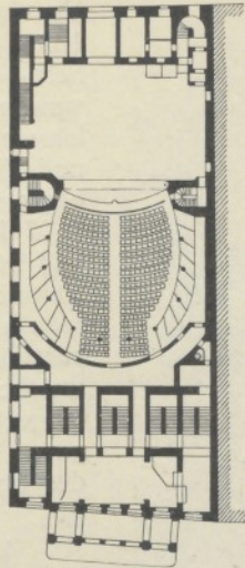
Abb. 483. Carl-Theater. Parterre. 1:1000.
