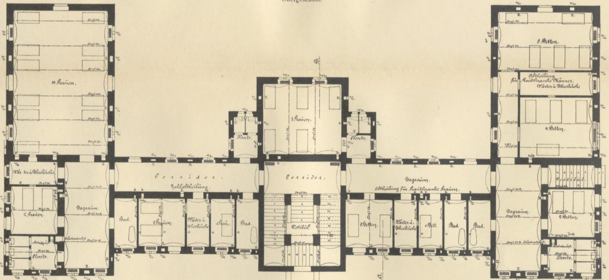
Erdgeschoss.
