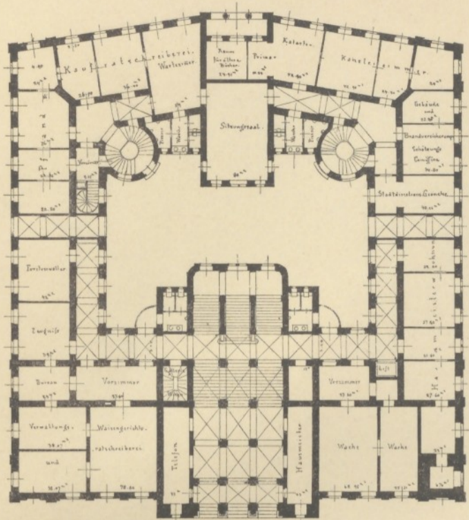
Erdgeschoss.
