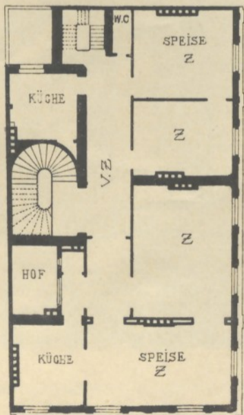
3. STOCK
