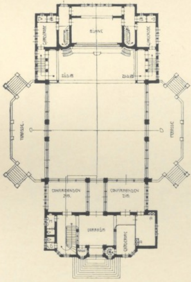
Erdgeschoss.
