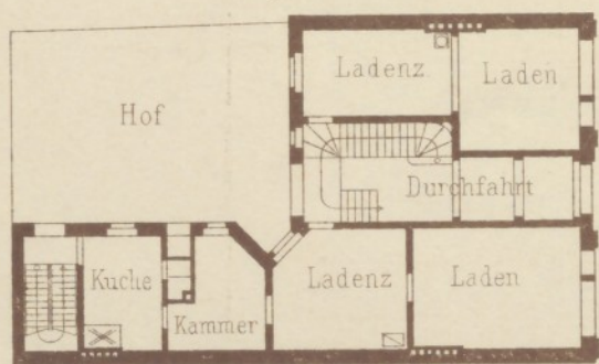
Erdgeschoss.
